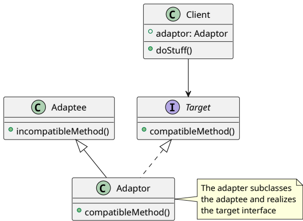
Figure 315: Diagram of the Class Adapter Pattern
